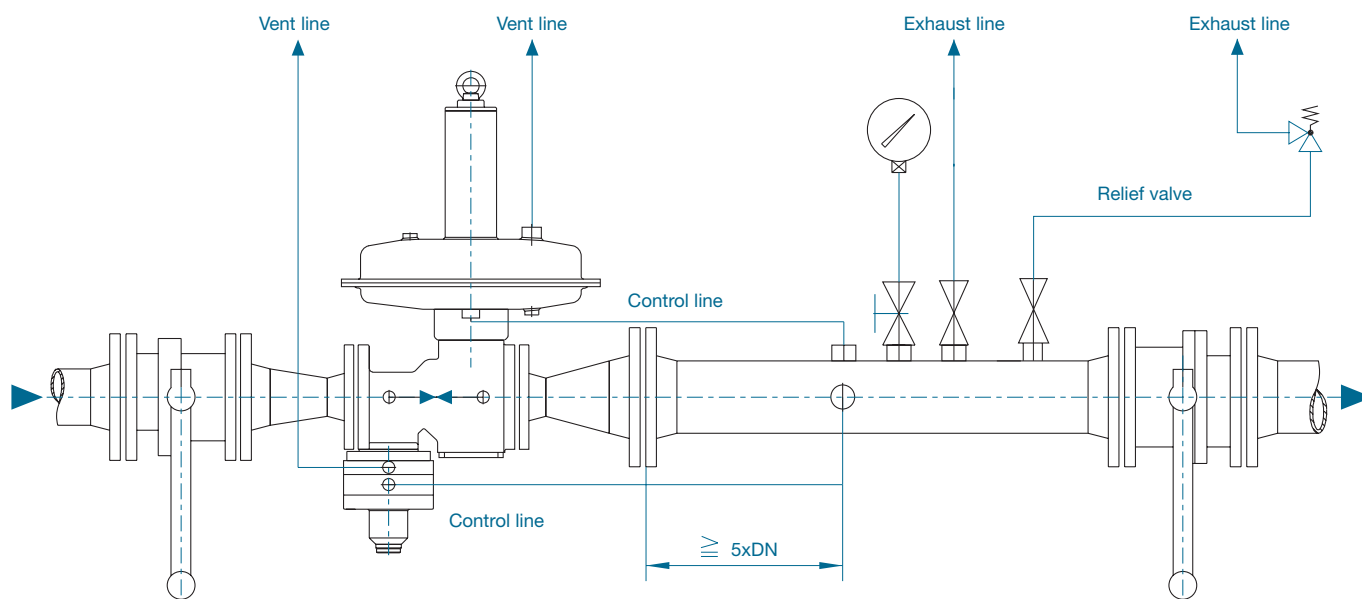
Typical installation
