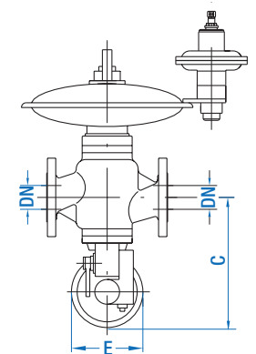
Regulator RB 4700 and SSV 8600
