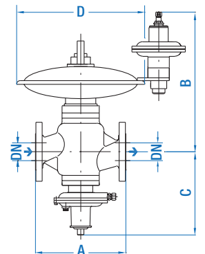
Regulator RB 4700 and SSV 8500
