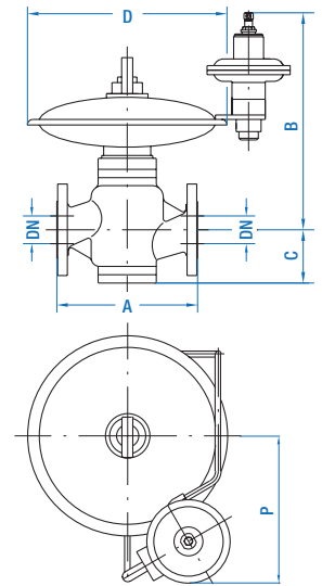
RB 4700 without SSV
